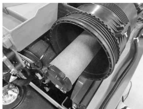
Air filter, inner screen element (replace only when necessary) 64713 (520) / 65229 (528/530))
